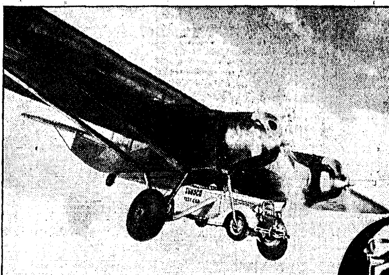
Flying from Floyd Bennett Field, N. Y., an Upper-Burnelli plane lifted a Ford car, suspended beneath the fuselage, a mile high into zero cold to prove the instant quick starting of Blue Sunoco Motor Fuel.
