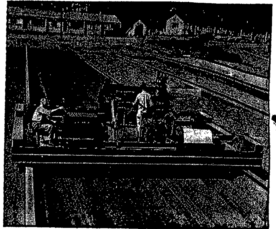
This large contraption is testing just one tractor tire. The new type machine, used for measuring the performance of rubber tires on farm tractors, is now in operation at the Department of Agriculture's proving ground at Alabama Polytechnic Institute, Auburn, Ala.
