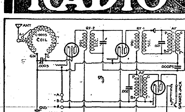
Three-Tube Receiver Using Low-Loss Doughnut Coil Coupler and Tuned Radio Frequency Transformer. Second Tube Is Refused So That It Amplifies Current at Both Radio and Audio Frequencies.
