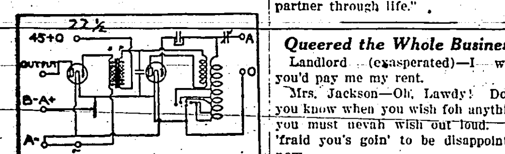
REGENERATIVE CIRCUIT
