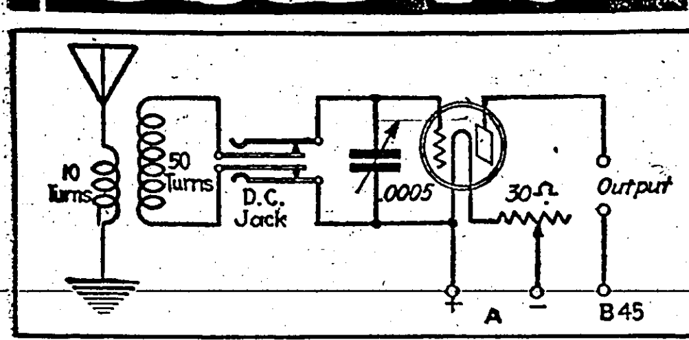
Diagram Showing How to Add a Stage of Radio Frequency to a Three-Tube Regenerative Set.
