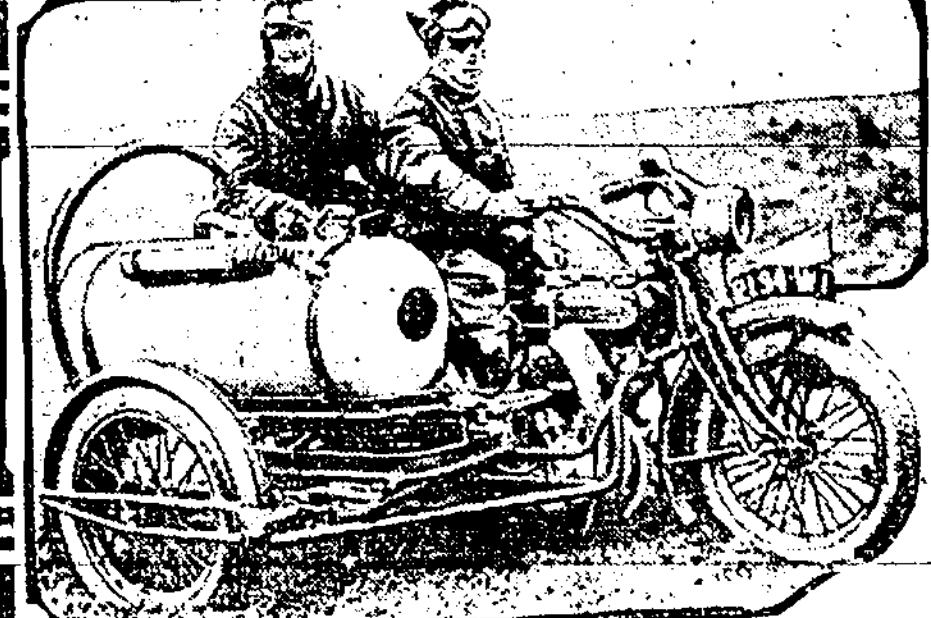
The French army has developed some new motor equipment that was demonstrated at recent maneuvers. The photograph shows a motorcycle war car.
