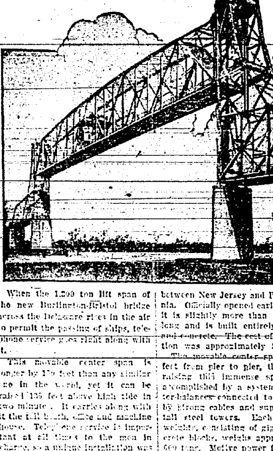
Thousand Ton 'Elevator' on Bridge Takes Rides With Telephone Aboard
