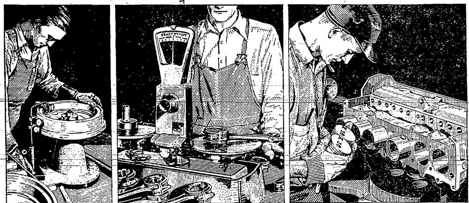
To achieve perfect fly-wheel balance, Chevrolet utilizes a special micrometer to balance every inch of the fly-wheel to a uniform thickness.
