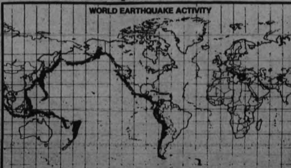
Most earthquakes occur in areas around the Pacific Ocean. The dark areas show the most active earthquake zones between 1961-1969.
