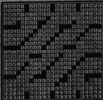
Crossword
