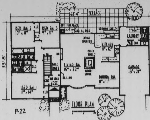
FLOOR PLAN — Living room, dining room and kitchen are open-planned around an open stove that is an attractive substitute for the conventional fireplace.
