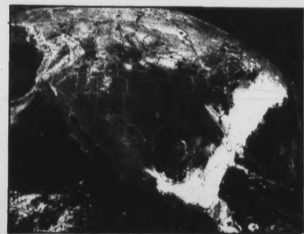
CLEAR SKIES Yesterday's weather satellite shows very few clouds over the nation. The best organized cloud band extends from northwestern Montana to northwestern California. Precipitation is confined mostly to this band. Other areas of clouds include southern Florida, the Carolinas and the northern tier of states. Clouds are also developing over Oklahoma. Snow covered ground extend from Maine through New York, Wisconsin and the Rockies to Washington.
