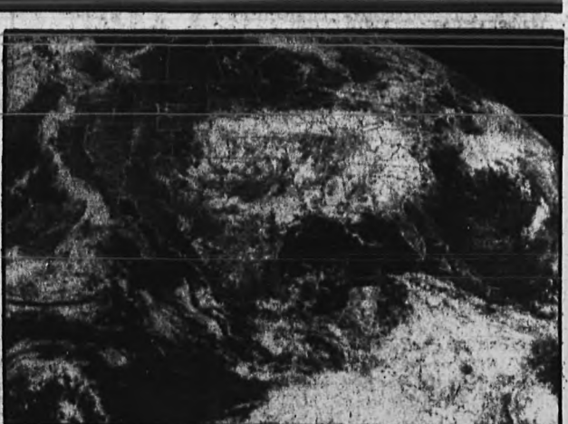
MAJOR CLOUD COVER — Yesterday's weather satellite photo shows a large swirl of clouds associated with a strong upper level storm system affecting a large portion of the nation. A band of layered clouds associated with this storm extend from the Southeast northward to the Lower Lakes and then westward to the Northern Plains. Strong thunderstorms are scattered along the Gulf Coast.
