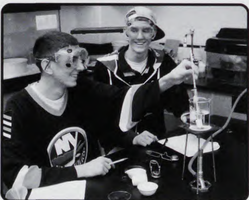
Below: Ben Hand and Will Rosen figure out a solubility curve.
