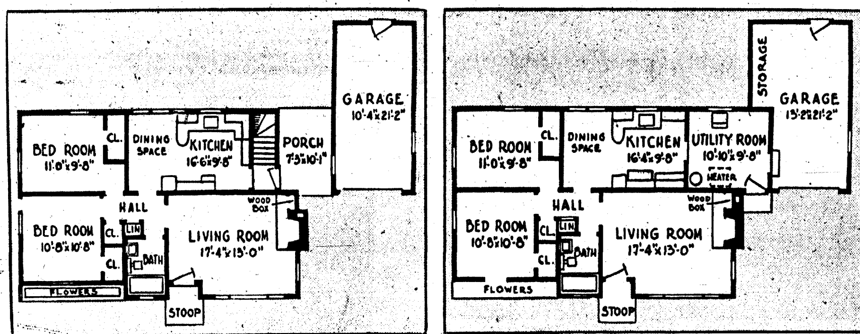
WHERE THE BASEMENT IS desired, the space given over to the utility room is occupied by basement stairs, breezeway to garage. WHICHEVER PLAN IS CHOSEN, the interior remains almost identical. Here, the basement has been omitted and a utility room installed.
