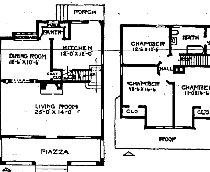
FIRST STORY PLAN. SECOND STORY PLAN.
