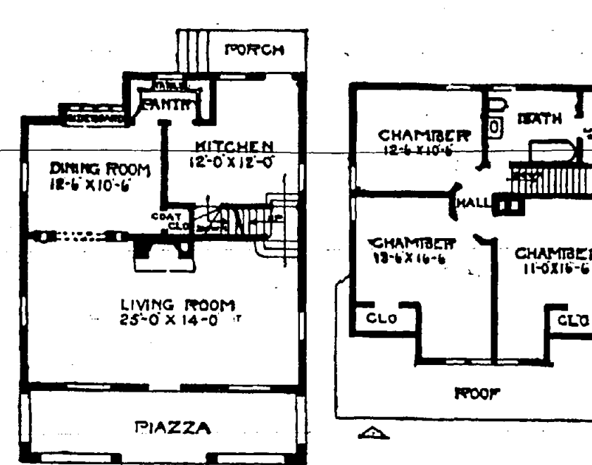
FIRST STORY PLAN. SECOND STORY PLAN.
