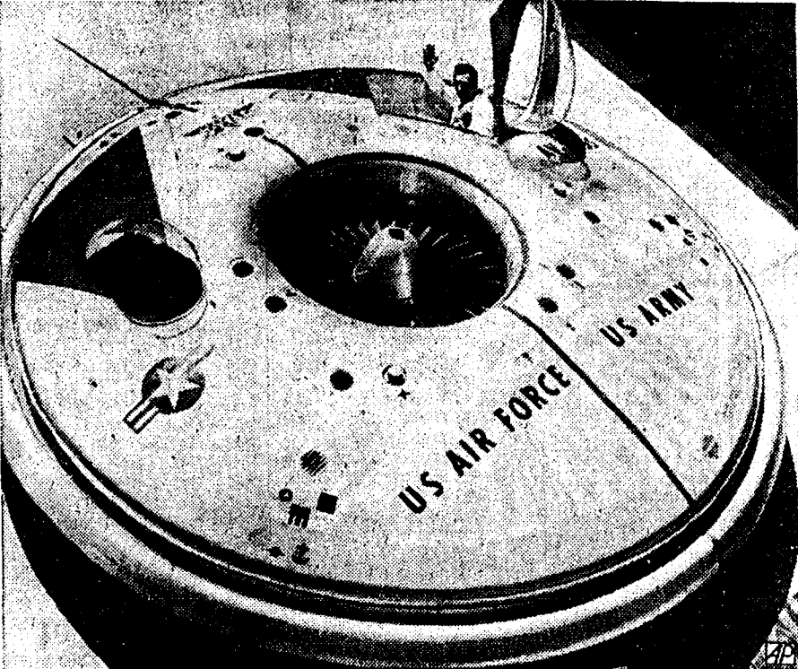
SAUCER DESIGNED TO FLY—The Defense Department released this photo Tuesday of a saucer-shaped research aircraft being developed for the U.S. Army and Air Force. The department said the craft is designed to take off and land vertically, using the air cushion principle, and to fly like a winged plane once it is in the air. A spokesman said the picture was made several months ago at the builder's (A. V. Roe Co.) plant in Canada. (U.S. Air Force Photo via AP)
