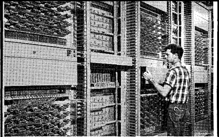
United Telephone switchman Joe Sato checks a "number group", part of the crossbar switching equipment going into service Sunday, July 12th.
